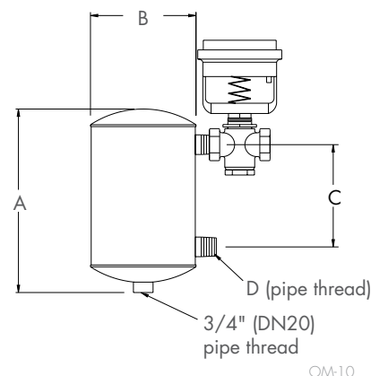
FIGURE 18-1: MULTIPLE-TUBE HUMIDIFIER SEPARATOR DIMENSIONS
