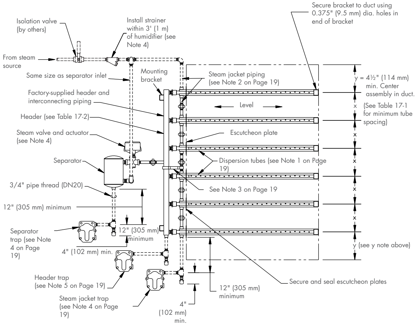
FIGURE 20-1: MULTIPLE-TUBE HUMIDIFIER WITH MAXI-BANK OPTION, TOTAL TUBE LENGTH LESS THAN OR EQUAL TO 45' (13.7 M) IN A DUCT, HORIZONTAL AIRFLOW
