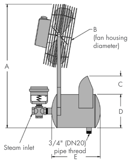
FIGURE 25-1: AREA-TYPE HUMIDIFIER
