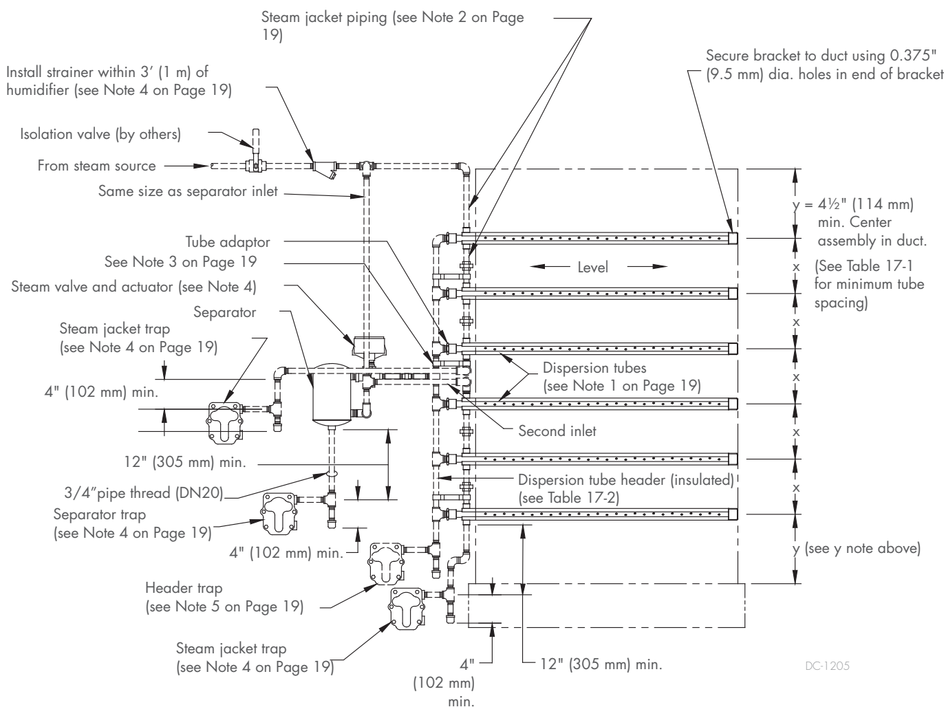
FIGURE 19-1: MULTIPLE-TUBE HUMIDIFIER WITH TOTAL TUBE LENGTH GREATER THAN 45' (13.7 M) IN AN AHU
