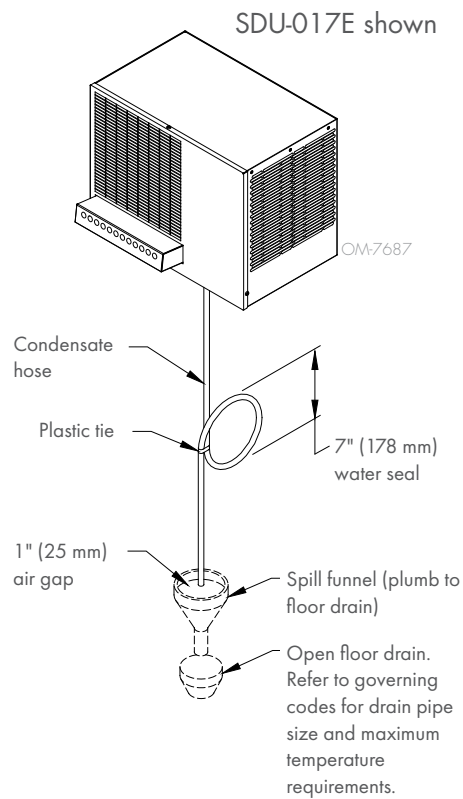
FIGURE 22-2: PIPING CONDENSATE TO DRAIN
