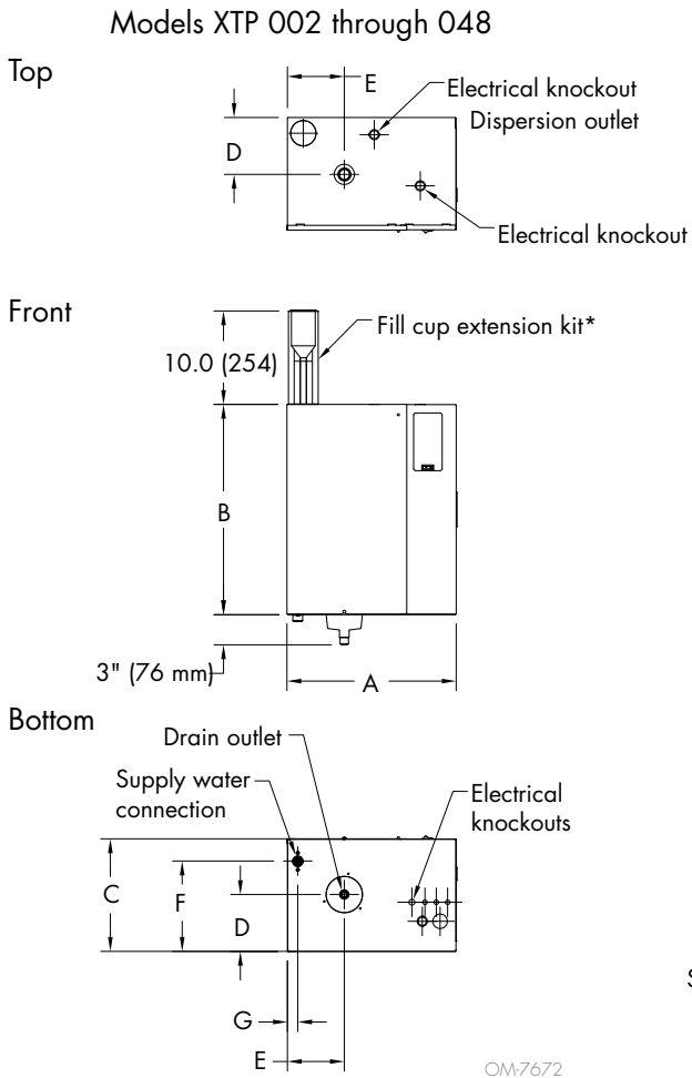
FIGURE 8-1: XT SERIES HUMIDIFIER DIMENSIONAL DRAWINGS
