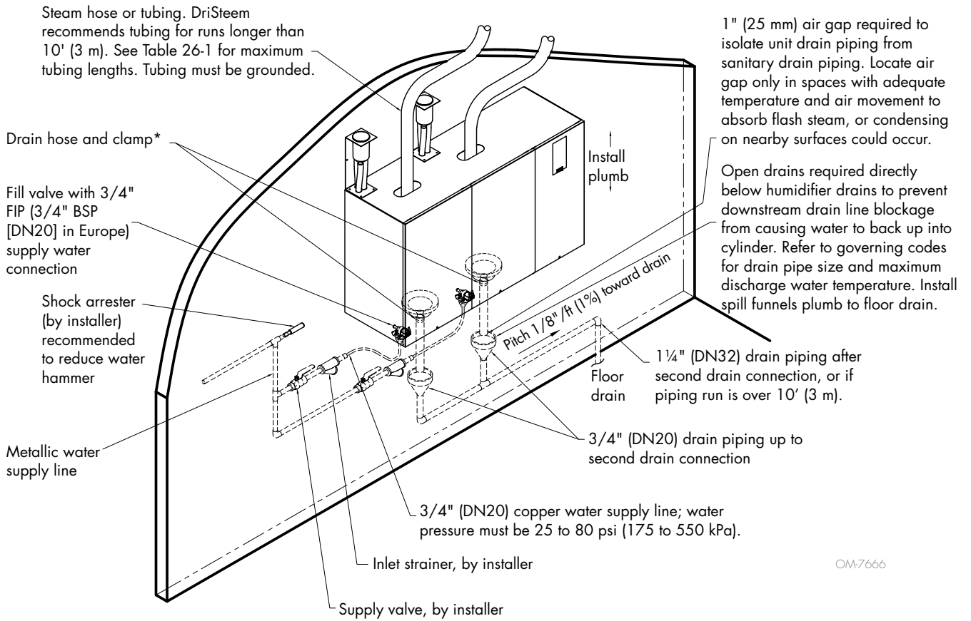
FIGURE 11-1: XT SERIES HUMIDIFIER FIELD PIPING OVERVIEW
