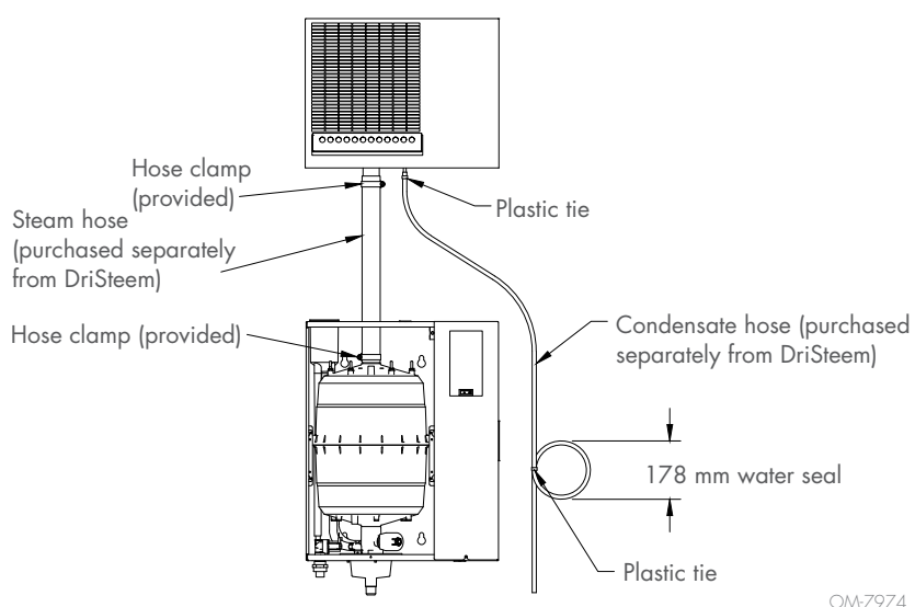
FIGURE 20-1: PIPING FROM XT SERIES HUMIDIFIER TO REMOTE XT STEAM BLOWER
