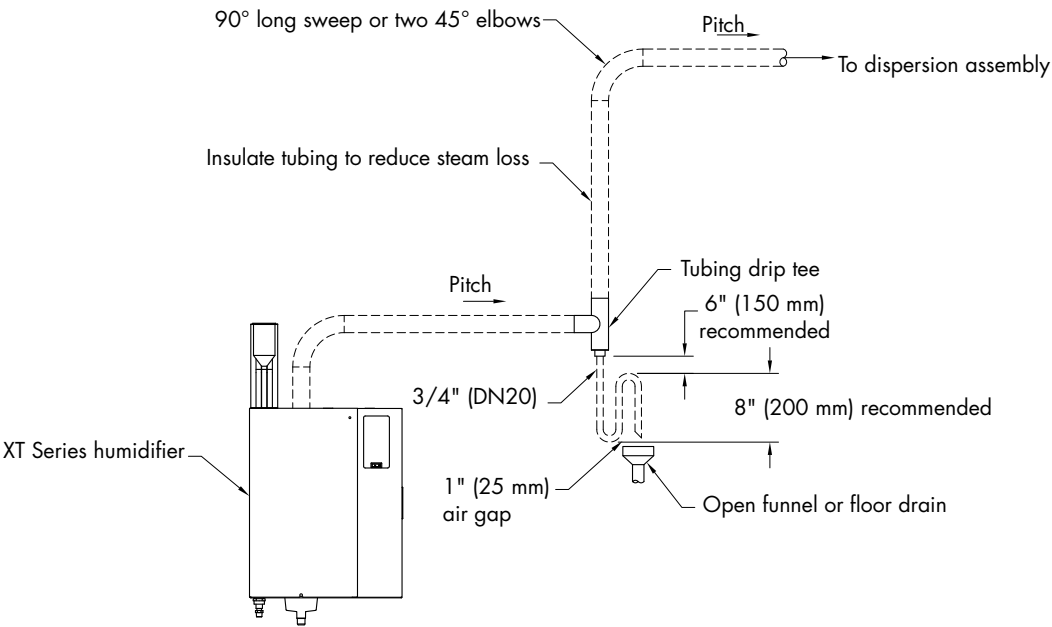
FIGURE 18-1: DETAIL OF VERTICAL RISER DRIPS
