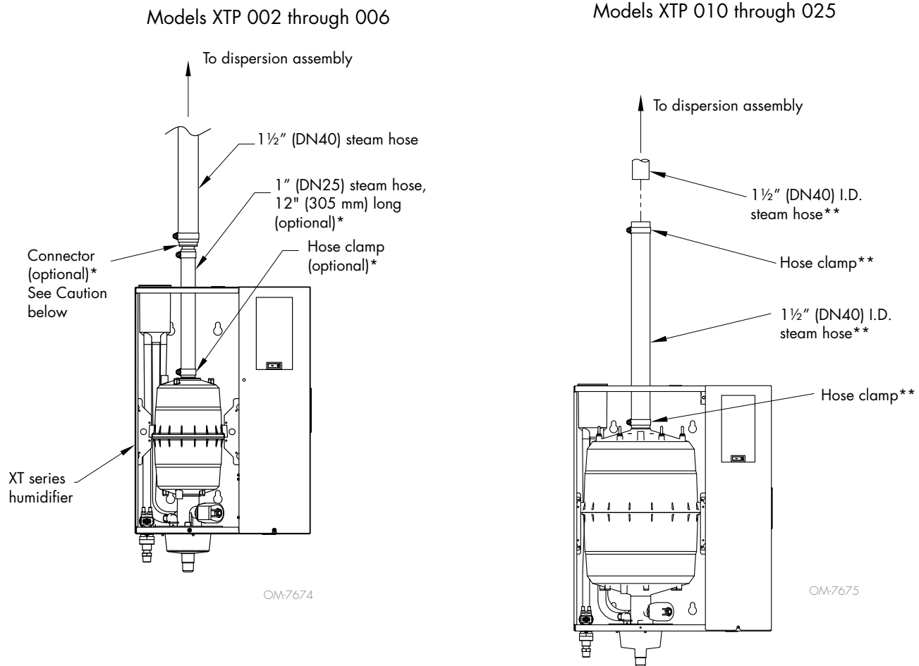
FIGURE 14-1: STEAM OUTLET CONNECTIONS, XTP MODELS 002 THROUGH 025
