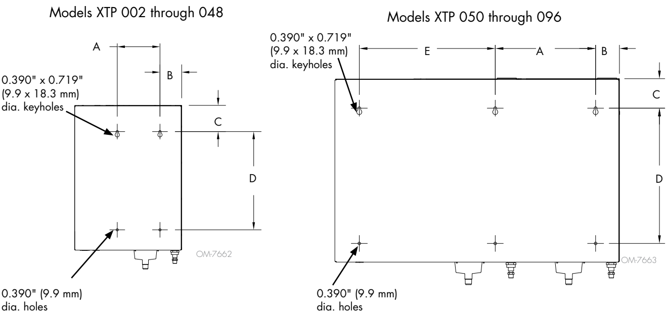
FIGURE 10-1: XT SERIES HUMIDIFIER MOUNTING KEYHOLE LOCATIONS
