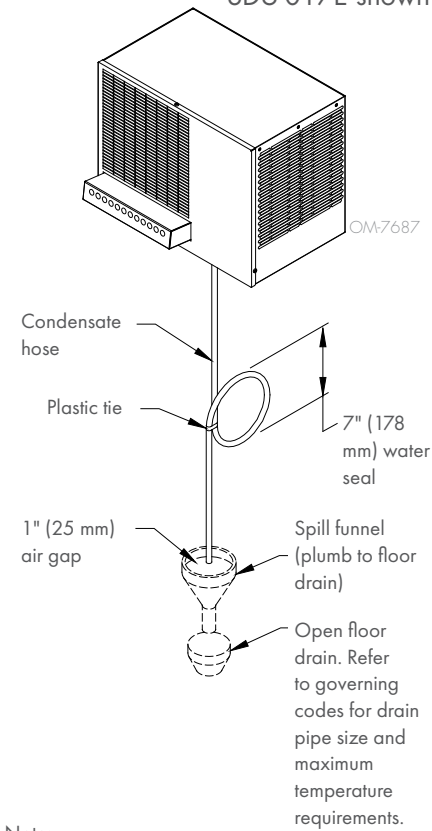
FIGURE 22-2: PIPING CONDENSATE TO DRAIN
