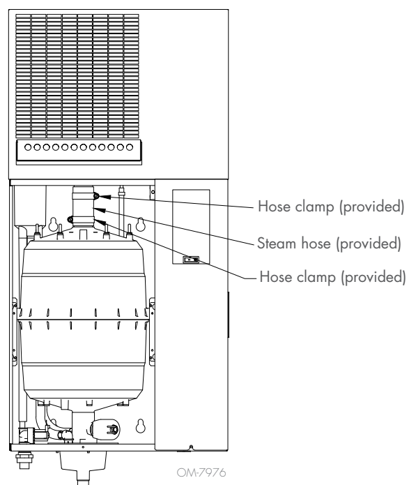
FIGURE 20-2: PIPING FROM XT SERIES HUMIDIFIER TO TOP-MOUNTED XT STEAM BLOWER
