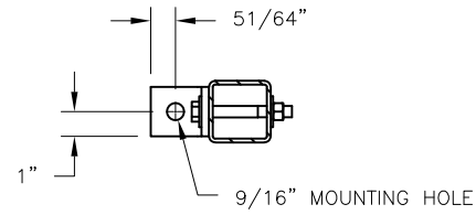
TOP VIEW OF DETAIL A
