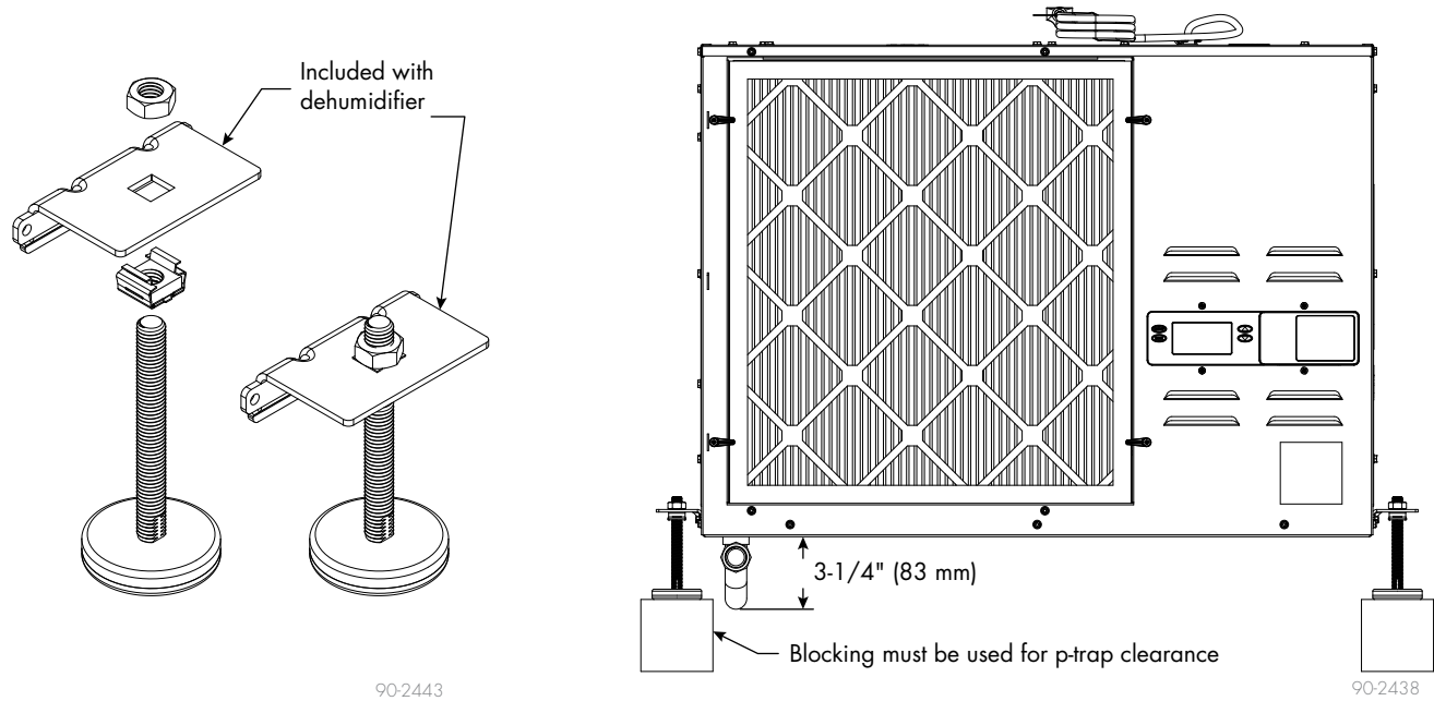
FIGURE 1-1: RL-14 FLOOR MOUNTING USE LEVEL FEET KIT (PART #601175)
