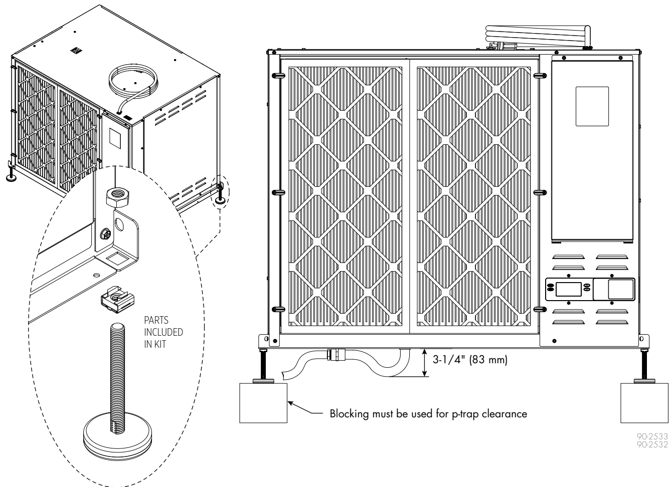
FIGURE 1-1: RL-31 FLOOR MOUNTING USE LEVEL FEET KIT (PART #601175)
