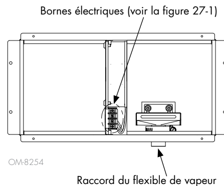
FIGURE 30-1 : RACCORDS DU FAN PACK XTR
