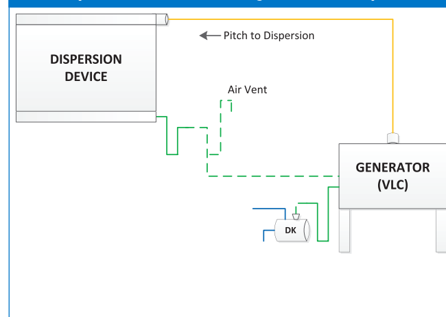
#11: Dispersion device with integral return - Vaporstream
