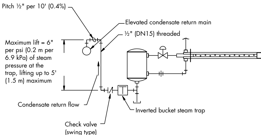
FIGURE 68-1: ELEVATING CONDENSATE
