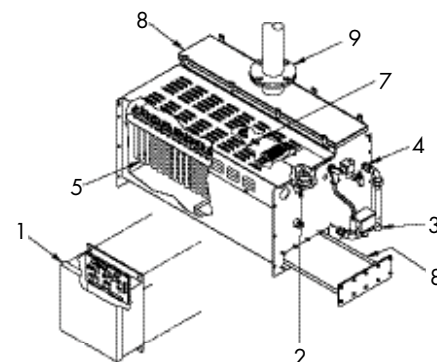
FIGURE 43-1: VAPORSTREAM ELECTRIC SYSTEM
