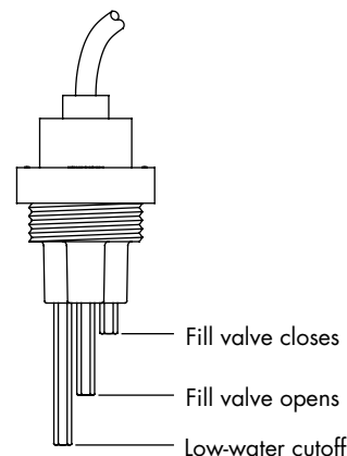
FIGURE 53-3: DETAIL OF CONDUCTIVITY PROBE
