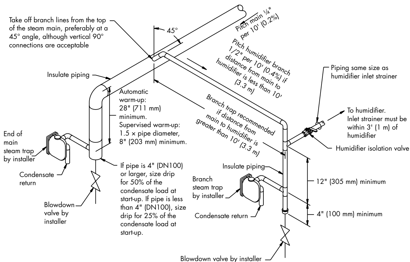
FIGURE 67-1: PIPING FROM BOILER TO HUMIDIFIER
