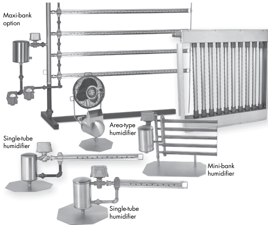
FIGURE 48-1: STEAM INJECTION HUMIDIFIERS
