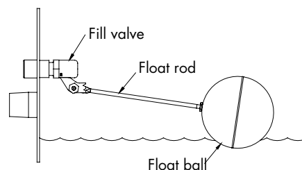
FIGURE 45-3: UNIVERSAL WATER LEVEL CONTROL
