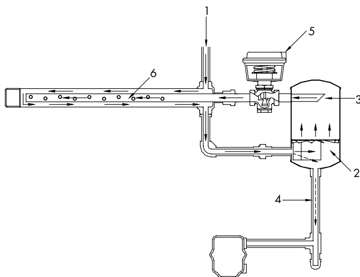
FIGURE 50-1: STEAM INJECTION PRINCIPLE OF OPERATION
