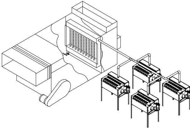
FIGURE 41-1: MULTIPLE STEAM GENERATORS AND AN ULTRA-SORB DISPERSION PANEL INSTALLED IN AN AHU
