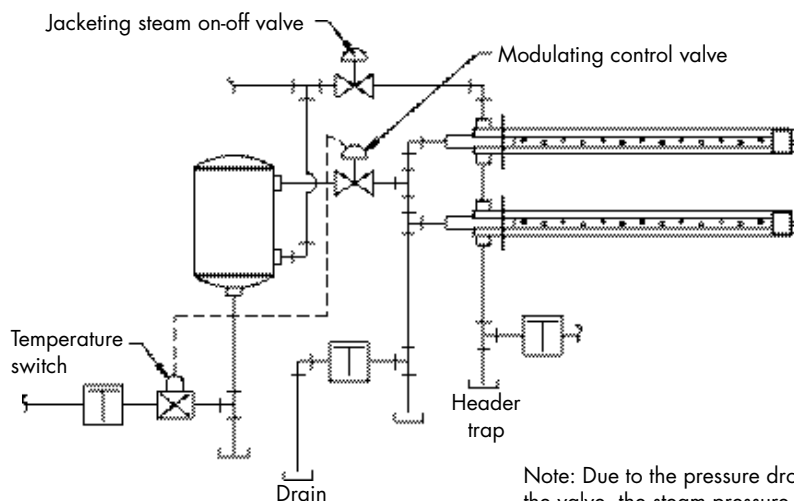
FIGURE 70-1: DIVIDED HUMIDIFYING STEAM PATH
