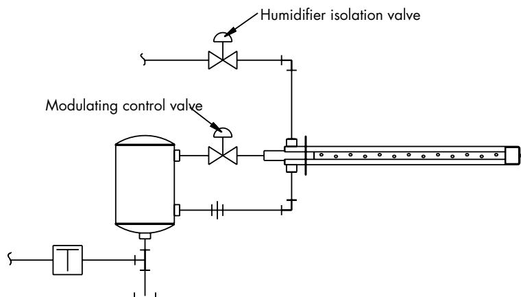
FIGURE 69-1: SINGLE HUMIDIFYING STEAM PATH
