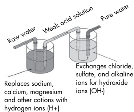
FIGURE 37-2: TWO-TANK DI SYSTEM
