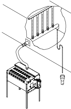
FIGURE 41-3: STEAM GENERATOR AND A SINGLE DISPERSION TUBE INSTALLED IN A DUCT
