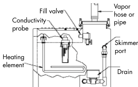
FIGURE 53-3: DETAIL OF CONDUCTIVITY PROBE
