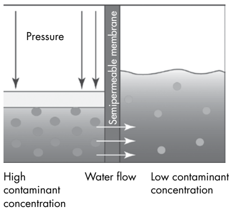
FIGURE 36-2: HOW REVERSE OSMOSIS FILTRATION WORKS
