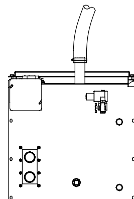
FIGURE 47-1: HOSE CONNECTION
