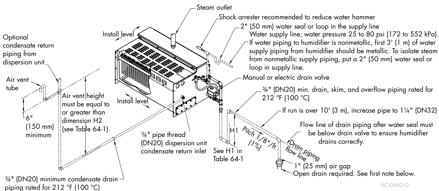
FIGURE 64-1: FIELD PIPING OVERVIEW, VAPORSTREAM WITH TAP/SOFTENED WATER
