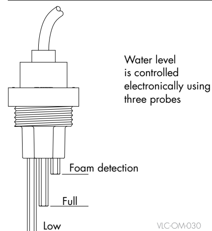
FIGURE 45-3: UNIVERSAL WATER LEVEL CONTROL
