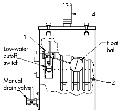
FIGURE 46-2: DI/RO WATER SYSTEMS
