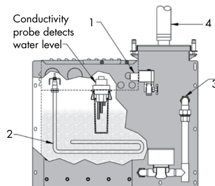
FIGURE 46-1: STANDARD WATER SYSTEMS
