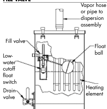
FIGURE 53-1: HUMIDIFIER WITH FLOAT-FILL VALVE
