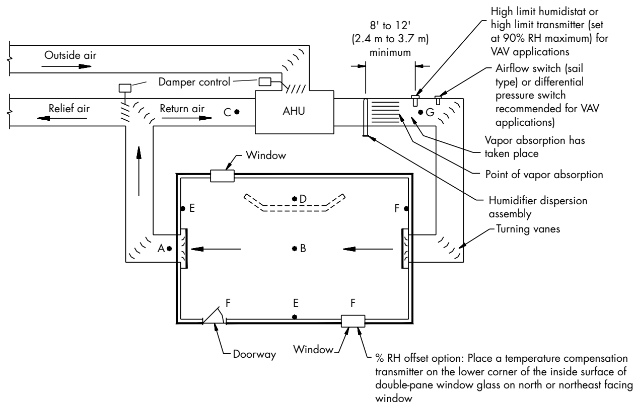
FIGURE 63-1: RECOMMENDED SENSOR LOCATIONS
