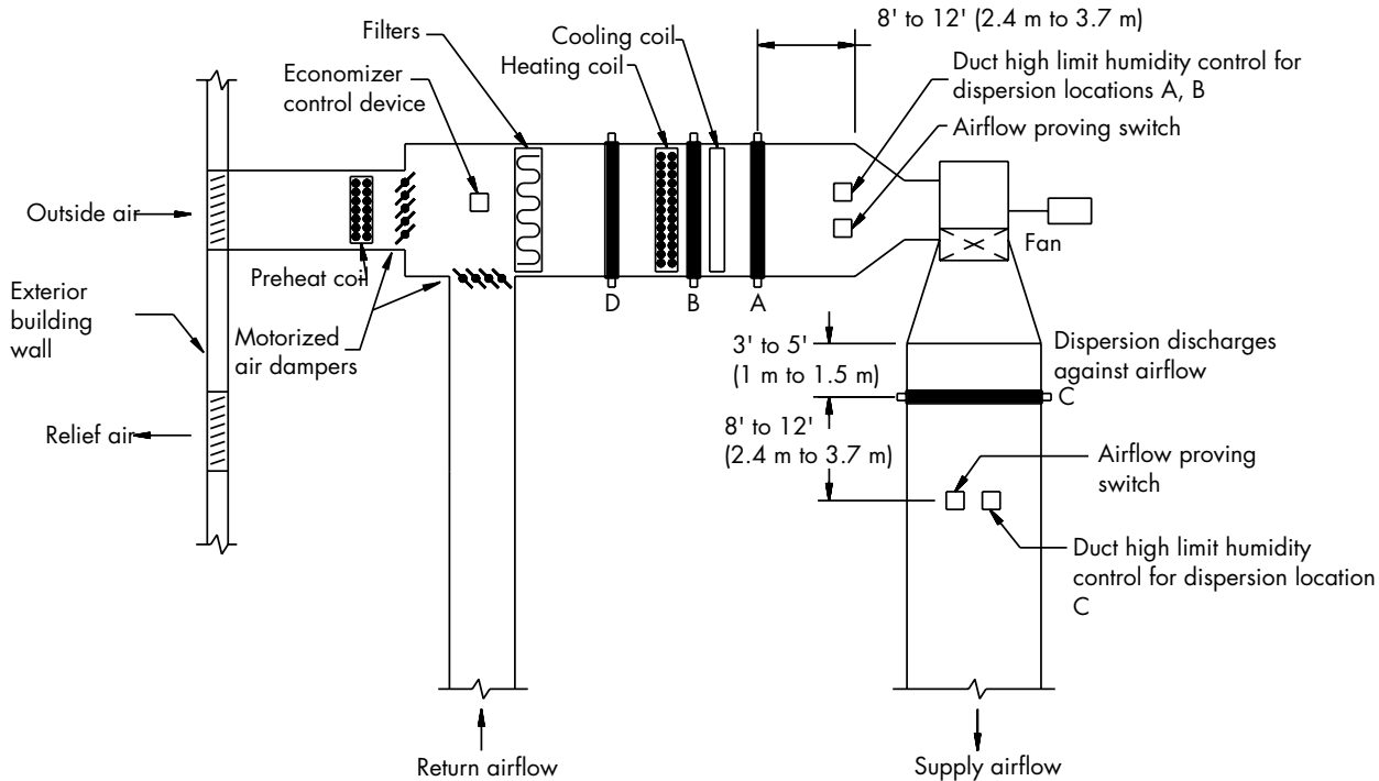
FIGURE 60-1: PLACING A DISPERSION ASSEMBLY IN AN AHU
