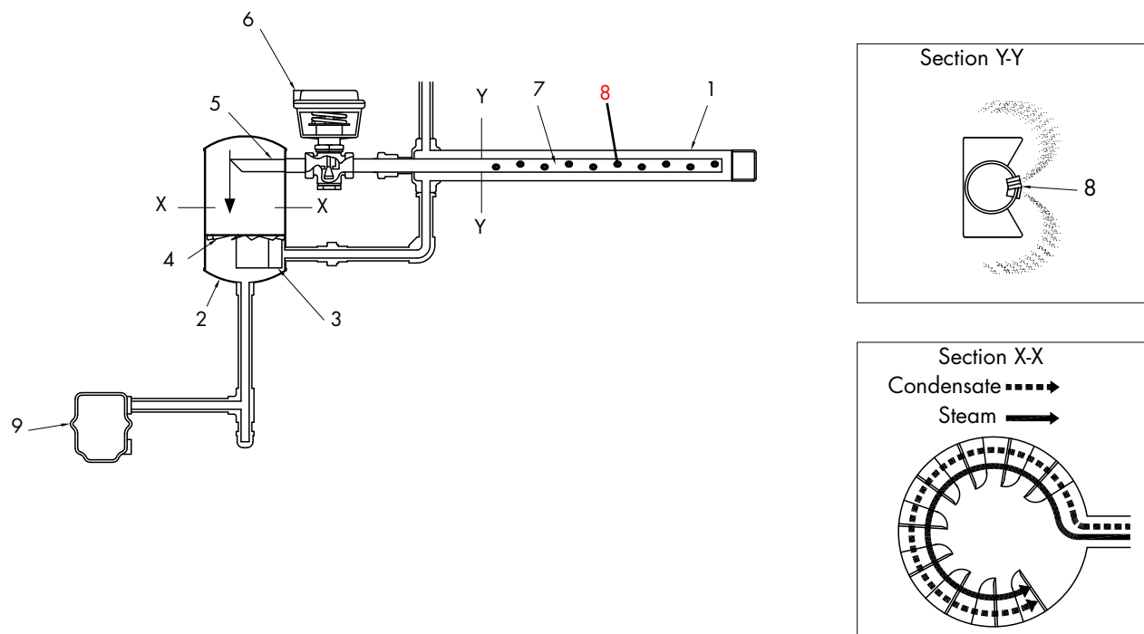
FIGURE 49-1: STEAM INJECTION COMPONENTS
