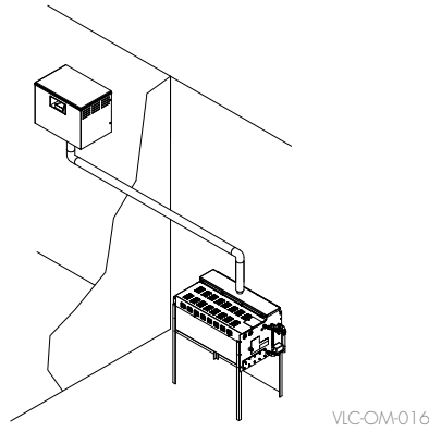
FIGURE 42-2: STEAM GENERATOR WITH A SPACE DISTRIBUTION UNIT INSTALLED DIRECTLY ABOVE
