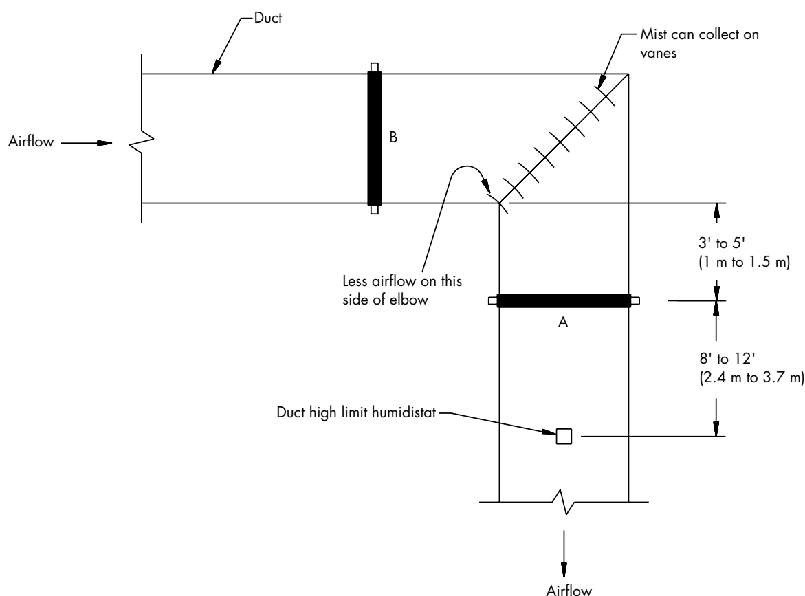
FIGURE 61-1: PLACING A DISPERSION ASSEMBLY NEAR AN ELBOW
