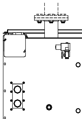
FIGURE 47-3: FLANGE CONNECTION
