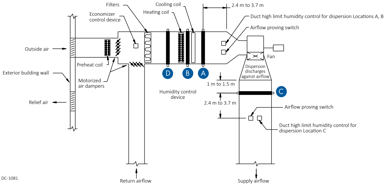
Figure 2: Placing a dispersion assembly in an AHU
