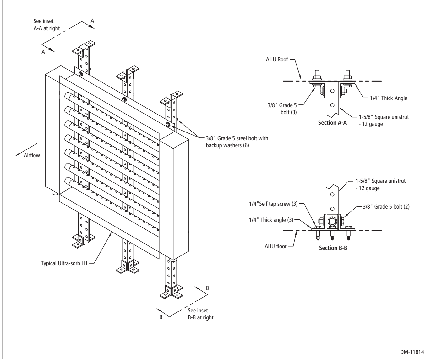
Figure 1-1: Ultra-sorb model LH seismic certification option installation in an air handling unit
