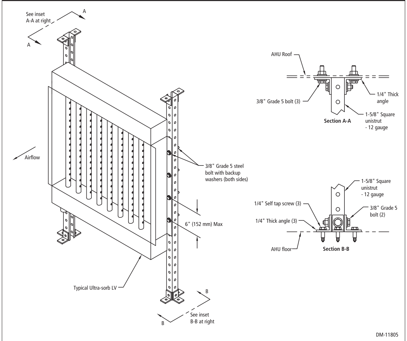
Figure 1-1: Ultra-sorb model LV seismic certification option installation in an air handling unit
