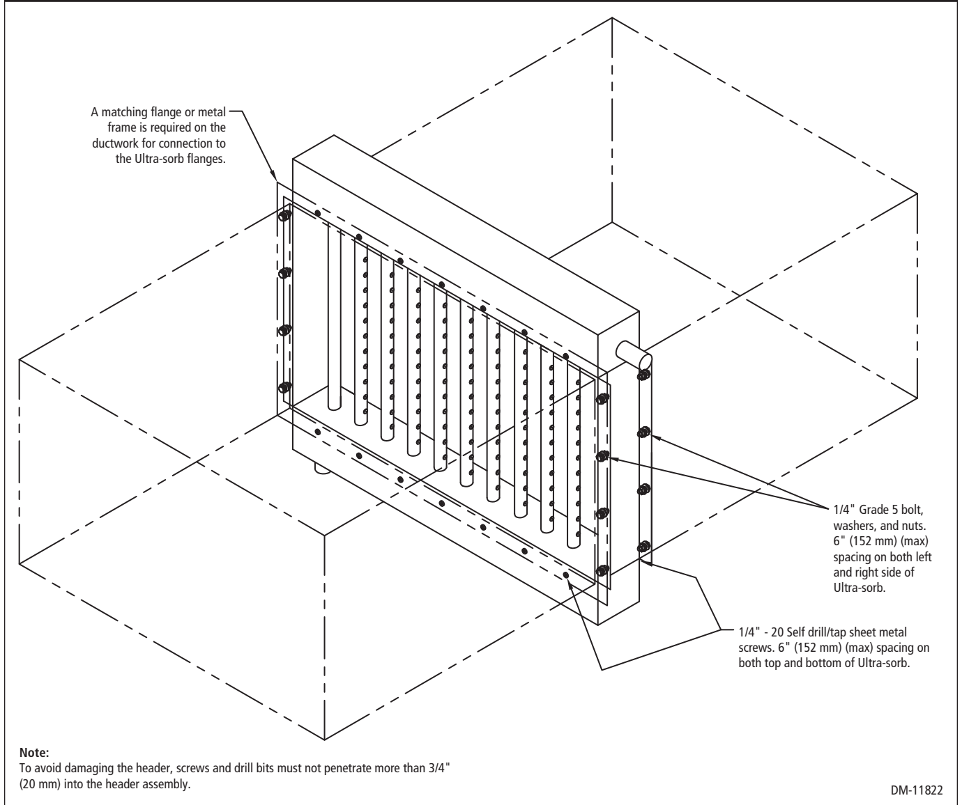
Figure 1-1: Ultra-sorb model LV seismic certification option installation in a duct
