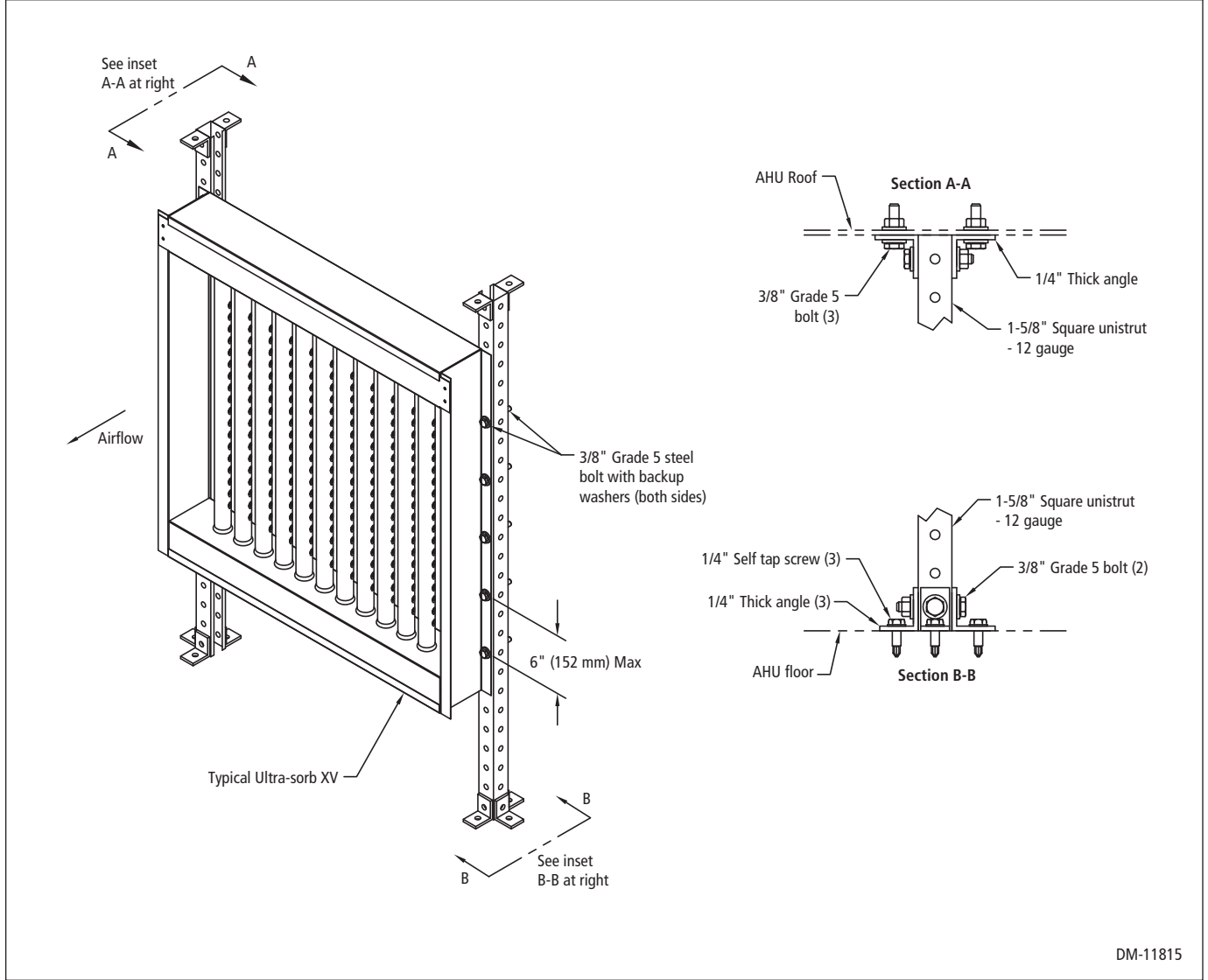
Figure 1-1: Ultra-sorb model XV seismic certification option installation in an air handling unit
