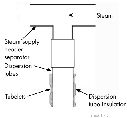
FIGURE 3-4: INSULATED TUBE DETAIL (HIGH-EFFICIENCY TUBE OPTION)
