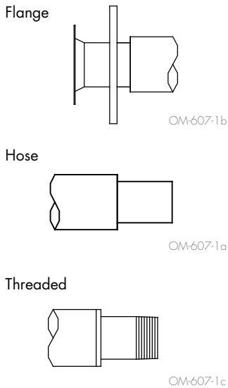
FIGURE 3-3: ULTRA-SORB MODEL LH STEAM INLET TYPES
