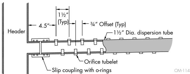
FIGURE 3-2: DISPERSION TUBE DETAIL
